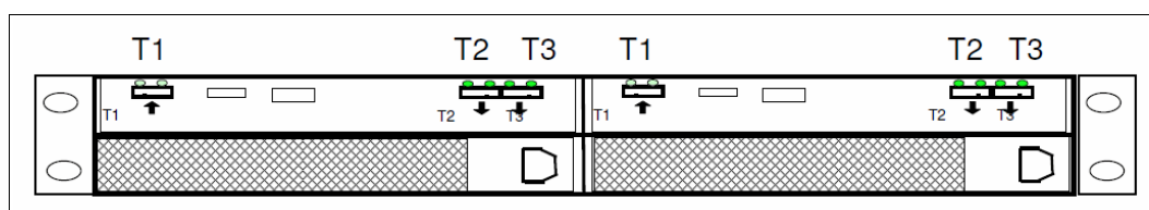
Figure 2-36 EXP24S SFF Gen2-bay drawer rear connectors
