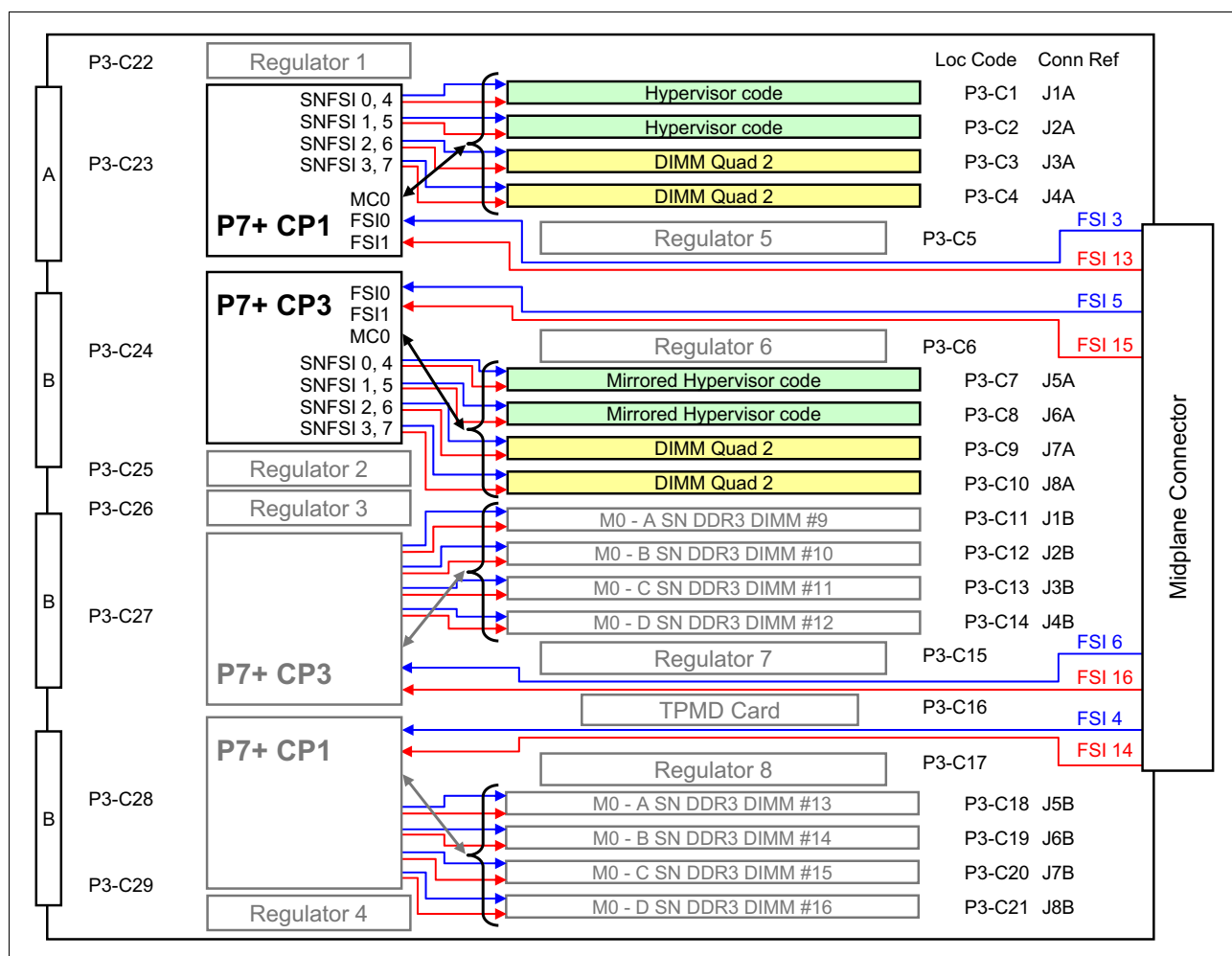
Figure 2-9 Active Memory Mirroring in a single CEC
