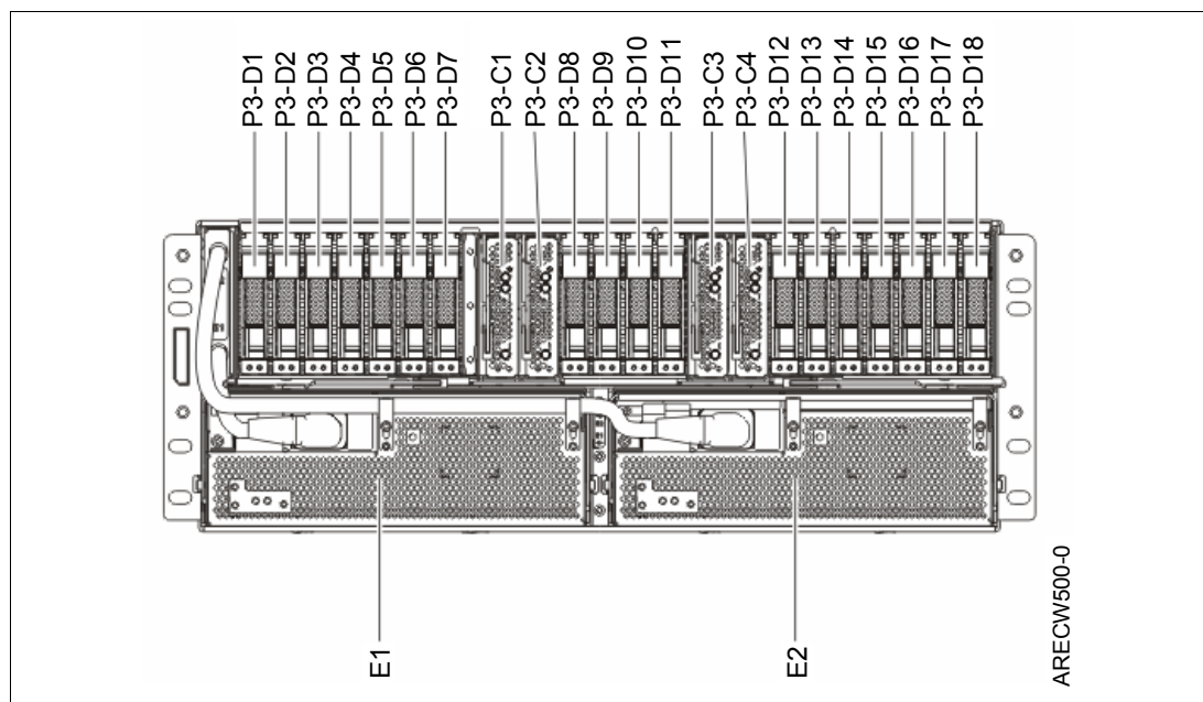
Figure 2-27 FC 5802 I/O drawer front view location codes
