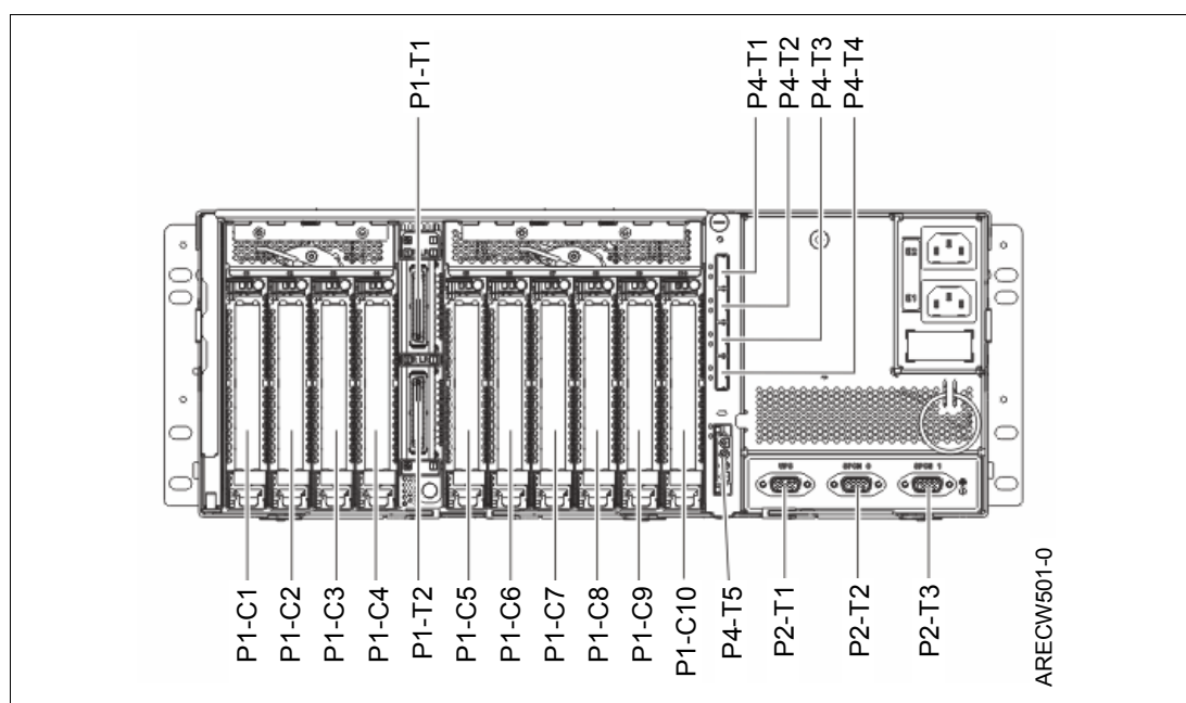
Figure 2-28 FC 5802 I/O drawer rear view location codes
