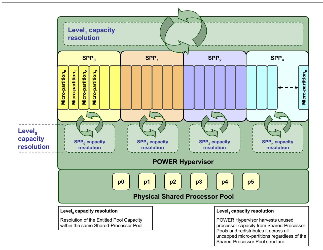
Figure 3-9 The levels of unused capacity redistribution
