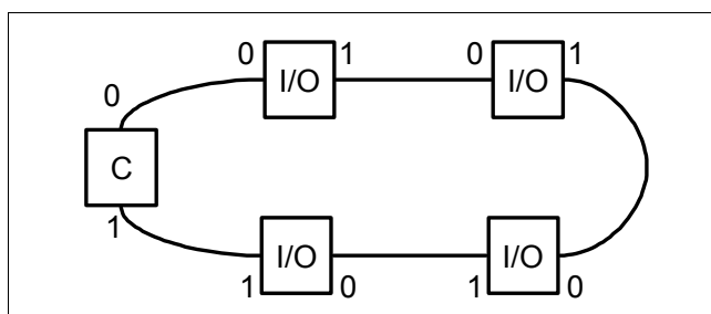
Figure 2-29 Typical 12X I/O loop port connections
