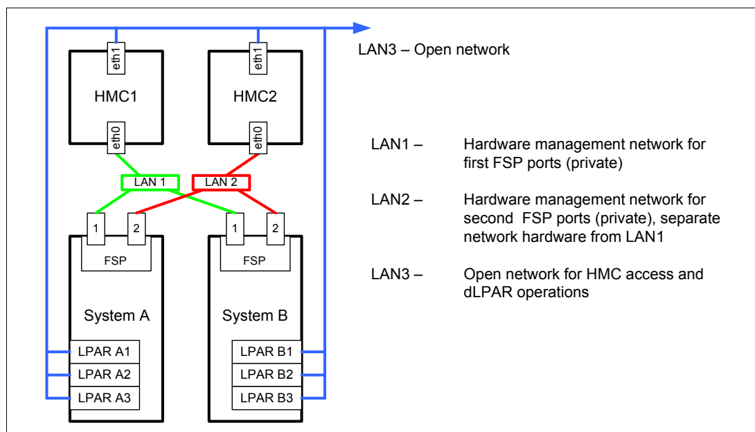
Figure 2-38 Highly available HMC and network architecture
