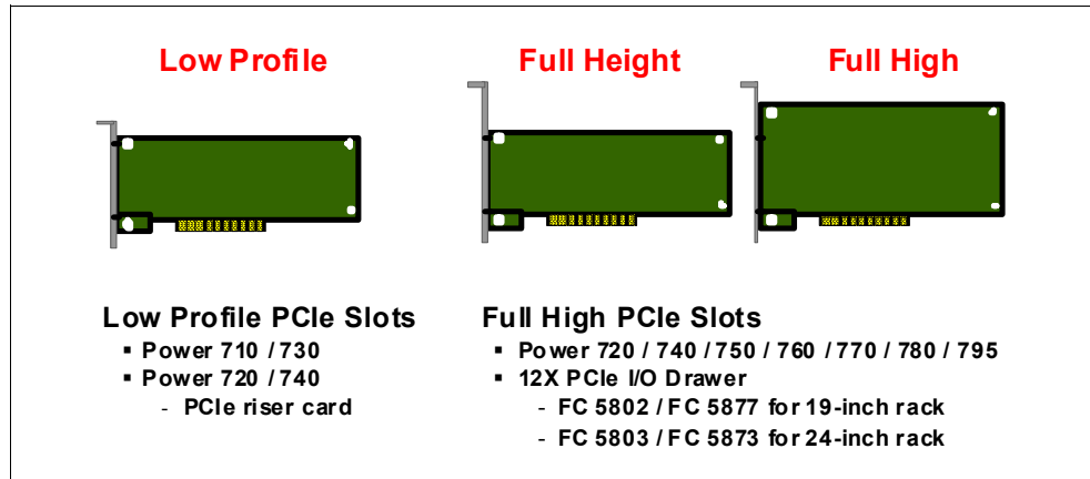
Figure 2-17 PCIe adapter form factors
