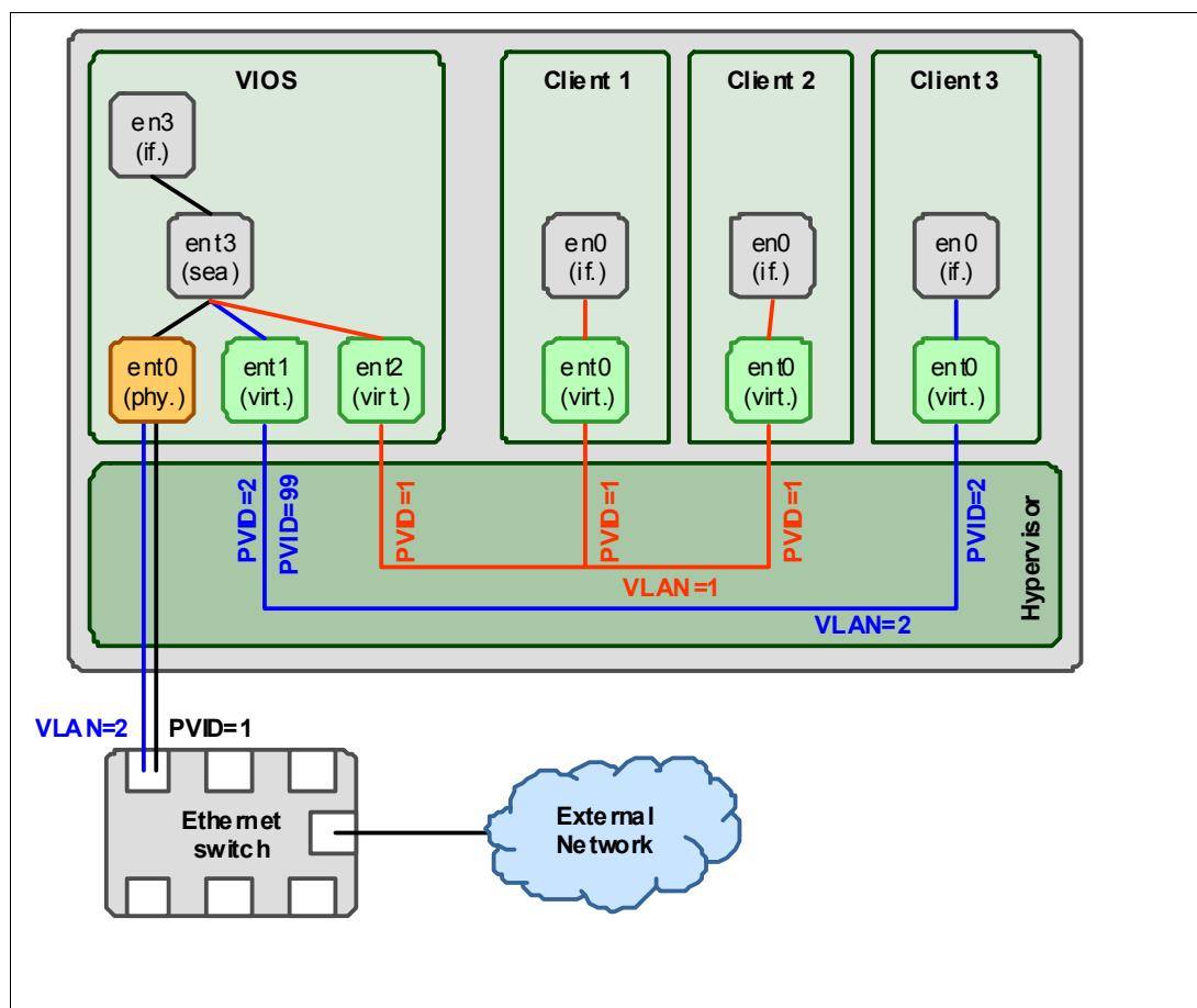
Figure 3-11 Architectural view of a Shared Ethernet Adapter
