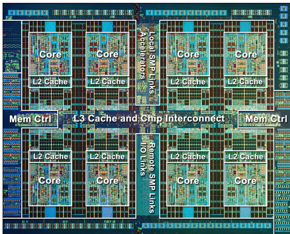
Figure 2-2 POWER7+ processor die with key areas indicated
