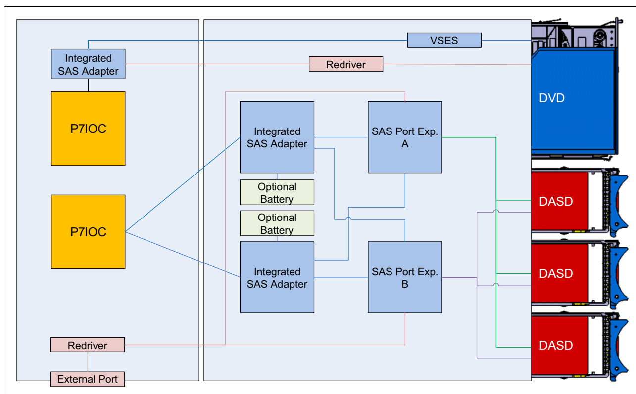
Figure 2-19 Internal SAS topology overview
