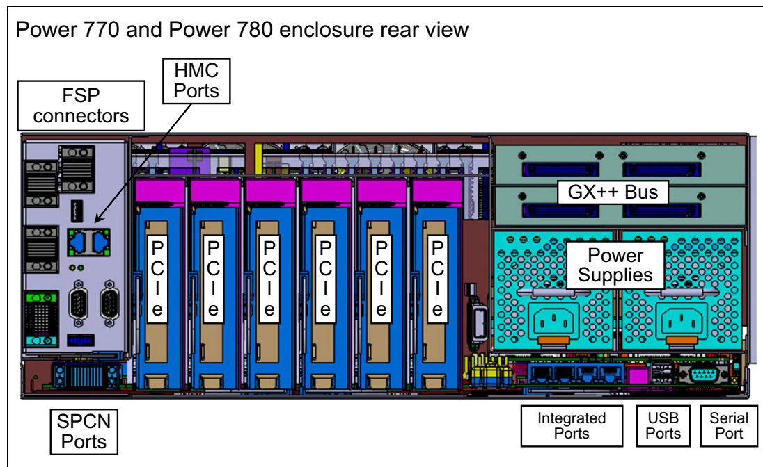
Figure 1-2 Rear view of the Power 770 and Power 780
