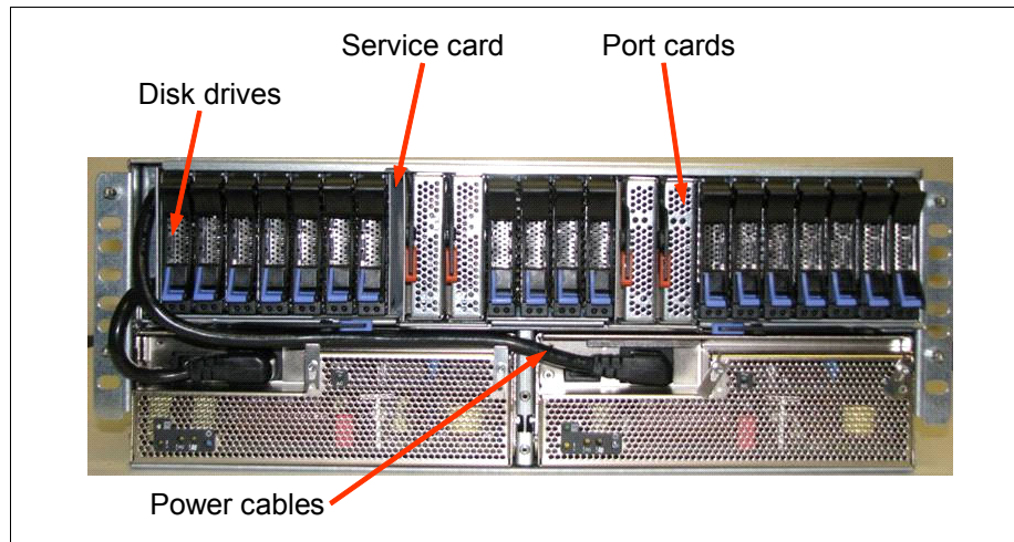
Figure 2-24 Front view of the 12X I/O Drawer PCIe
