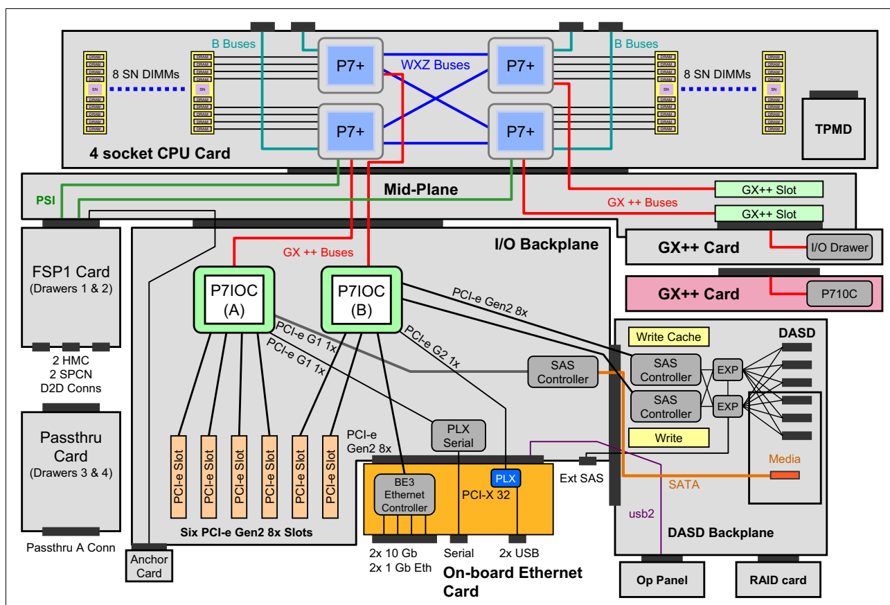
Figure 2-1 IBM Power 770 or 780 logical system diagram
