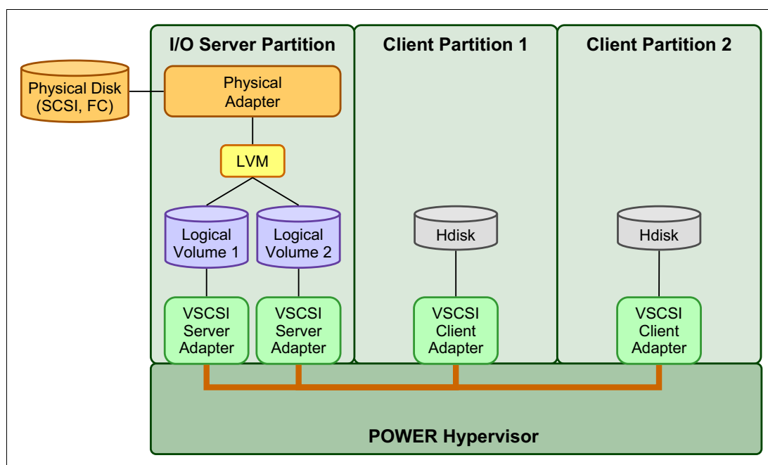
Figure 3-12 Architectural view of virtual SCSI
