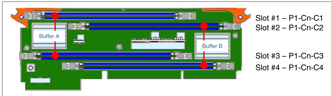
Figure 2-14 Memory riser card for the Power 710 and Power 730 systems
