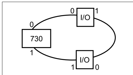
Figure 2-26 Typical 12X I/O loop port connections
