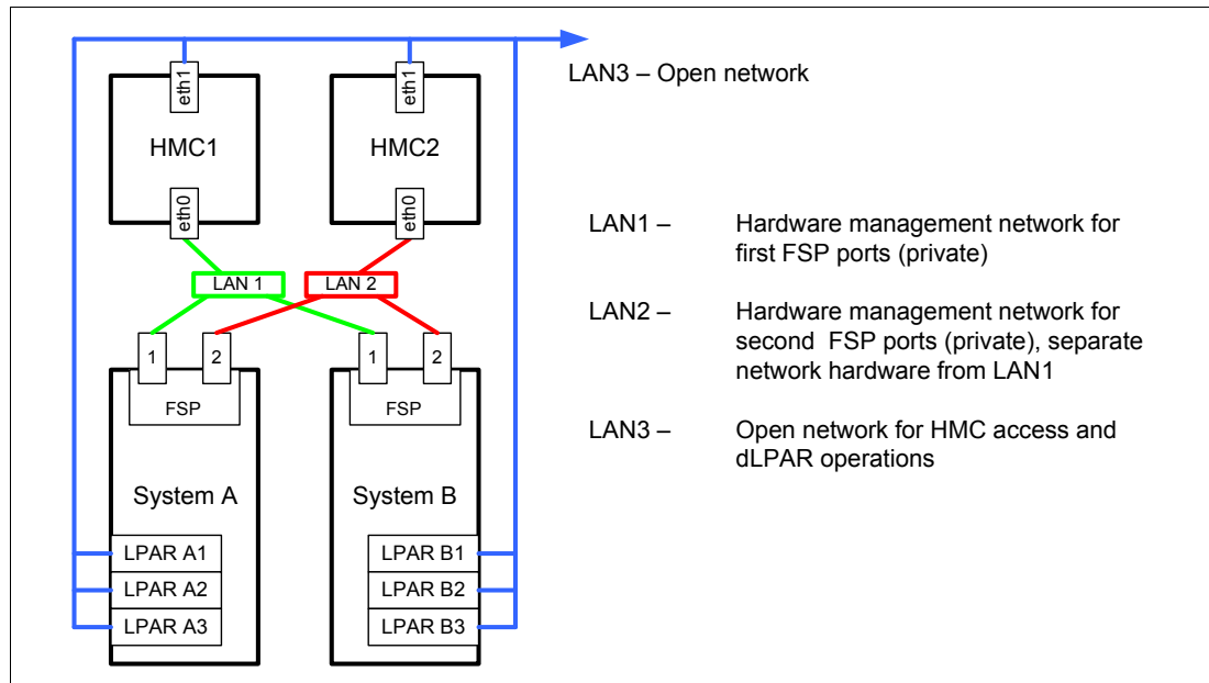
Figure 2-34 Highly available HMC and network architecture
