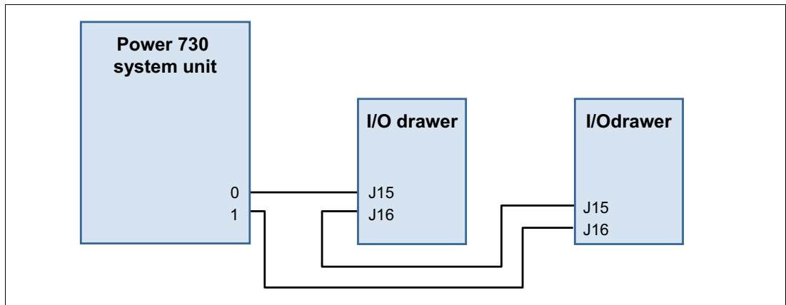
Figure 2-27 SPCN cabling example
