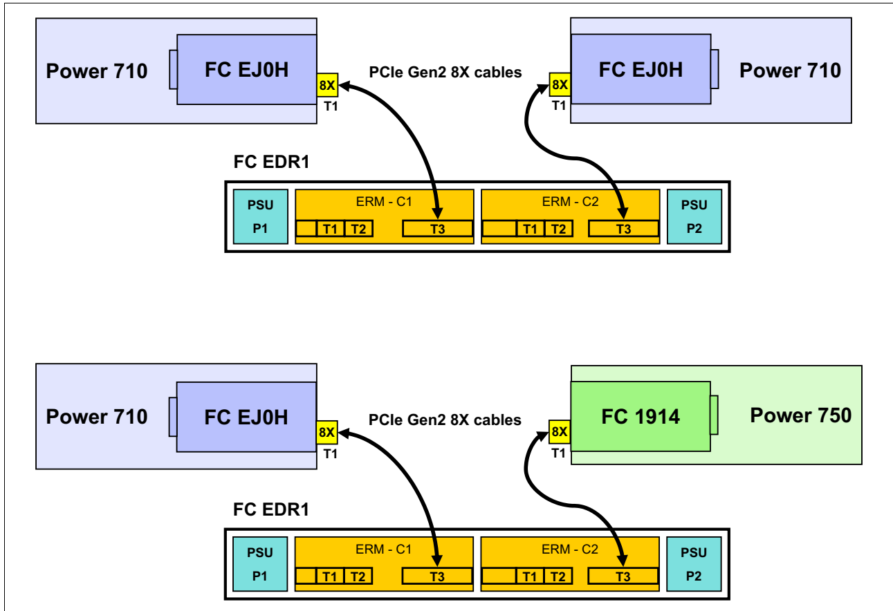
Figure 2-29 Connection between Power 710, an FC EDR1 drawer and a Power 750 server
